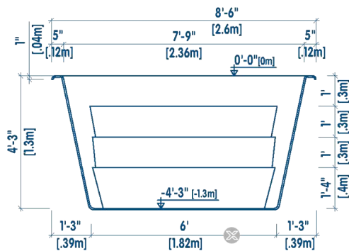
CORTE TRANSVERSAL | CROSS SECTION
